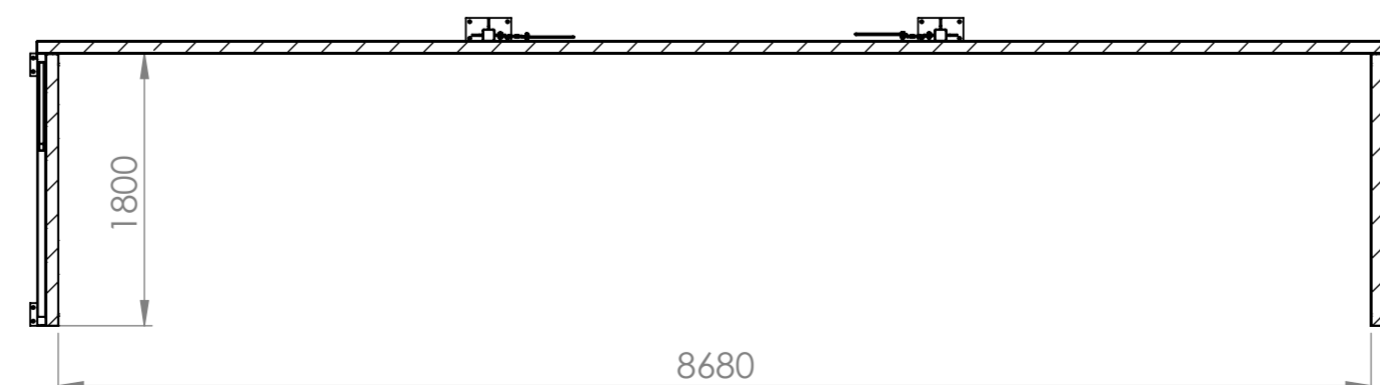
SECTION B-B
